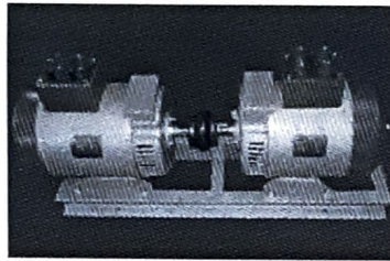
5HP DC Shunt Motor Coupled To 3 KVA Single Phase Alternator
