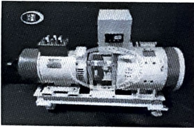
7.5 HP DC Shunt Motor with 5HP Alternator with Digital Tacho
